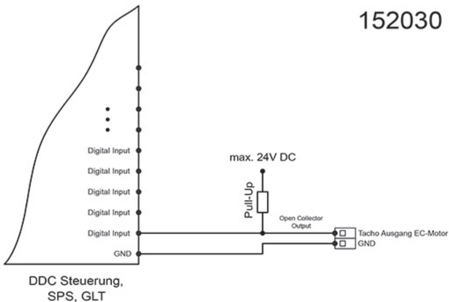
Tacho output (speed out) connected to control unit
